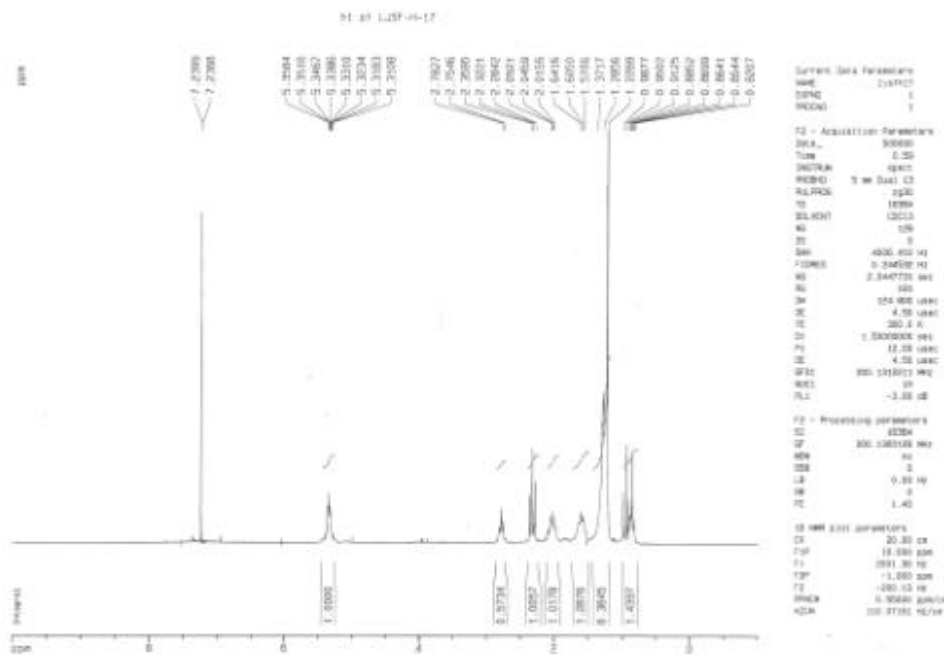
圖 4 : 1 H-NMR spectrum of compound II
